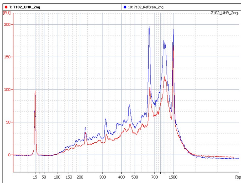
Figure 2. Bioanalyzer trace of SPIA cDNA product obtained from 2 ng of Human Brain and Universal Human Reference RNA using the DNA 1000 Labchip.
